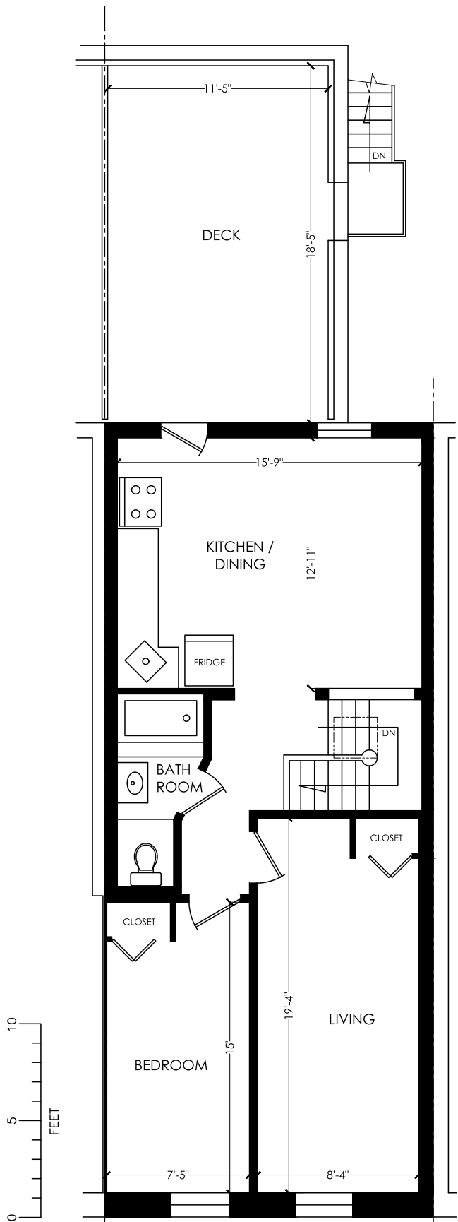
THIRD FLOOR FLOOR AREA: 696 SQ. FT.
