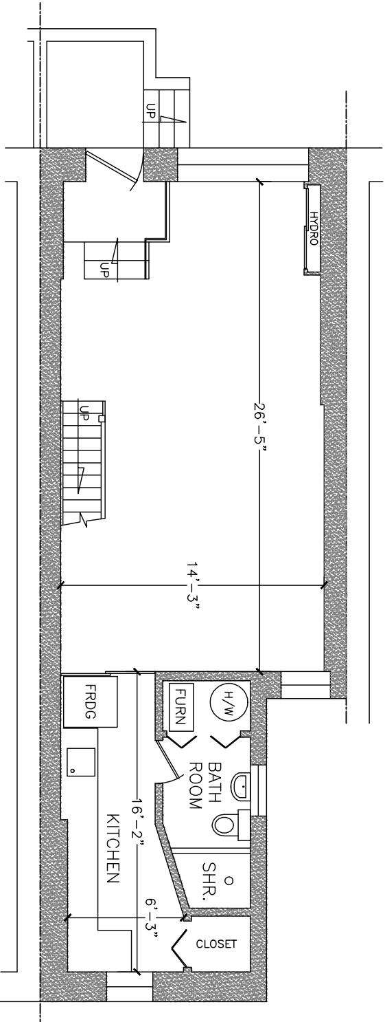
BASEMENT FLOOR AREA 692 SQUARE FEET
