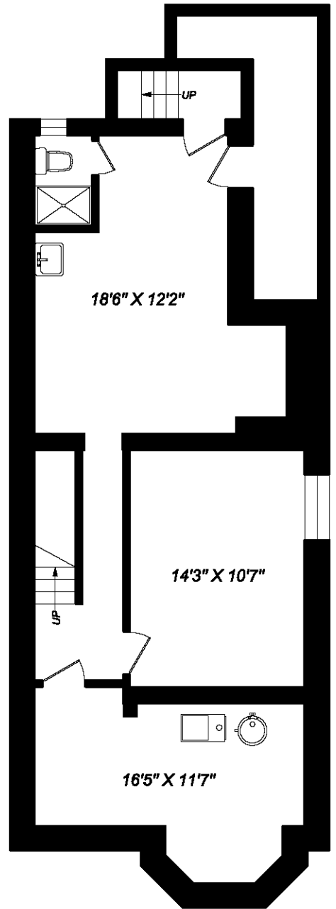
LOWER LEVEL 808 SQUARE FEET
